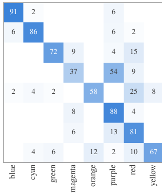
Static, occluded acc 73.0% (n=393)
