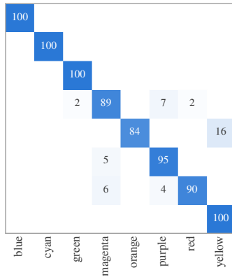
Moving, occluded acc 94.6% (n=386)
