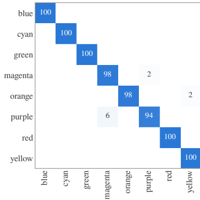
Static, no occluder acc 98.7% (n=393)
