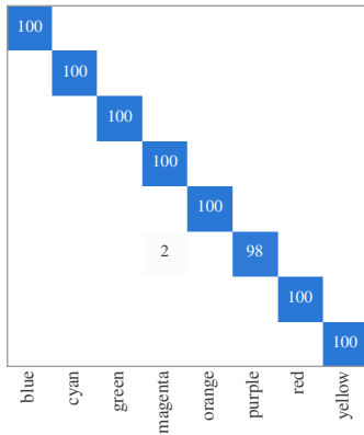
Moving, no occluder acc 99.7% (n=390)
