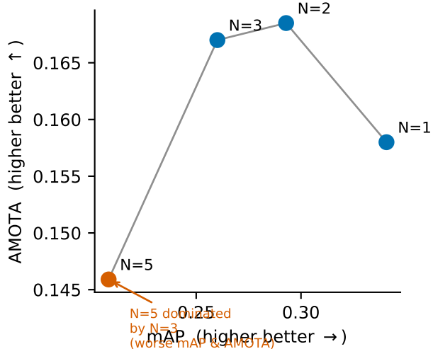
mAP-AMOTA trade-off
