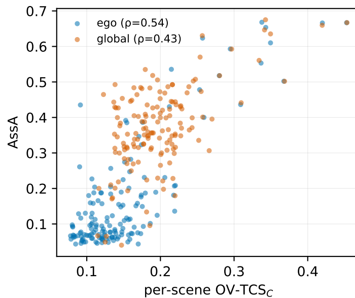
OV-TCS vs GT-track MOT metrics — nuScenes val, per scene
