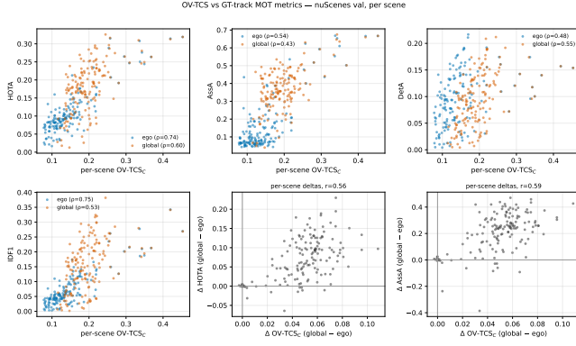
Figure 2: Per-scene OV-TCS vs. GT-based MOT metrics (nuScenes val, 150 scenes per arm). OV-TCS, computed without any ground-truth identities, tracks the association-quality axis (HOTA/AssA/IDF1) and not the detection axis.
