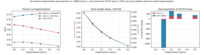
Figure 1: Controlled fragmentation ( p = 0 \rightarrow 0.5 , nuScenes val150, \sim 20k tracks per level; detections frozen). mAP is constant by construction and measurement. OV-TCS falls monotonically, and the decomposition shows the drop is carried entirely by L_{\text{norm}} while the stability factor ( 1 - \text{CSR} ) rises — the case that breaks stability-only metrics (Sec. 5.3).
