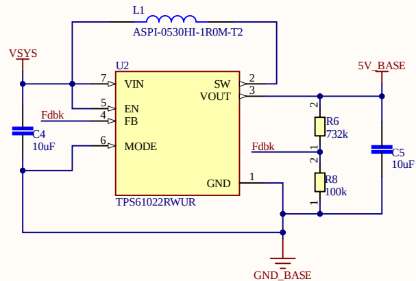
5V Reg
