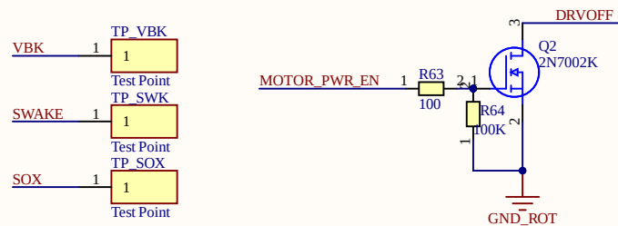
Motor Controller
