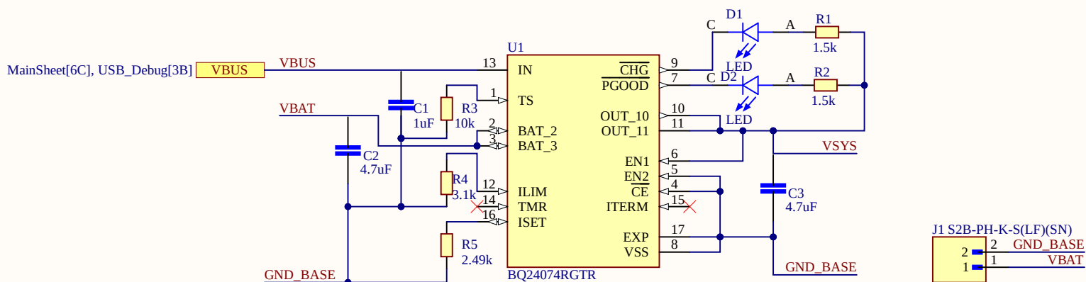
Charger / Power Path
