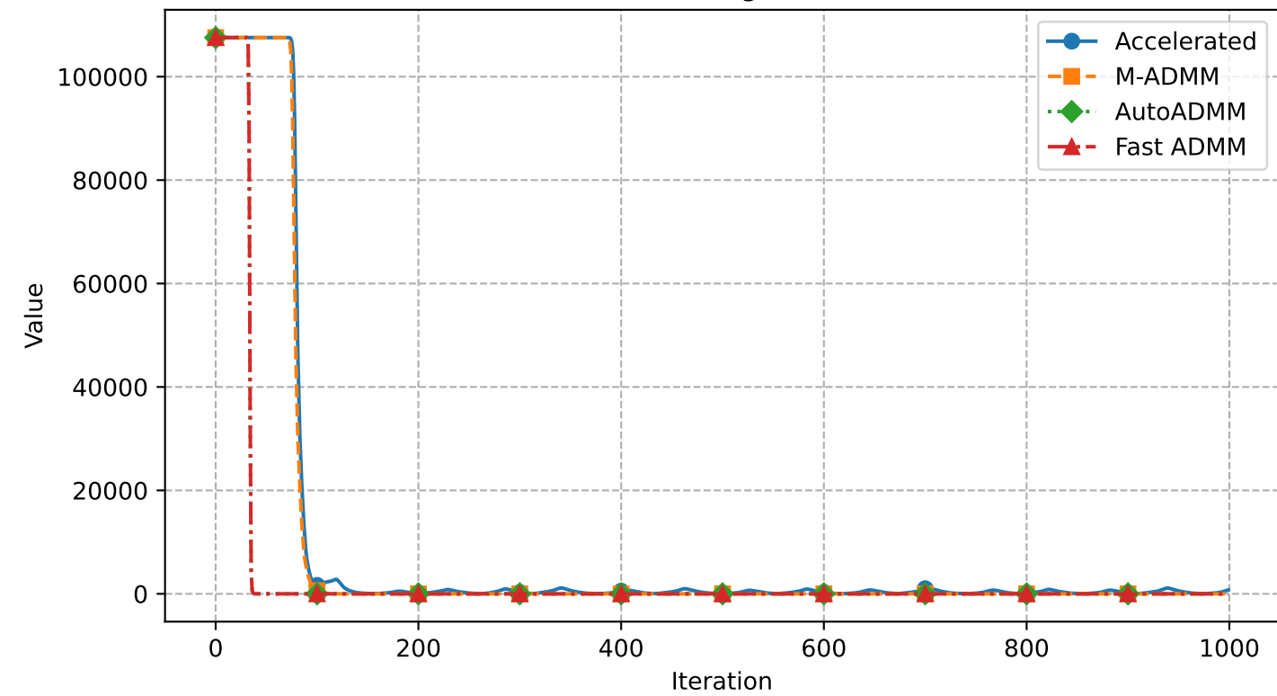
Dual Residuals
