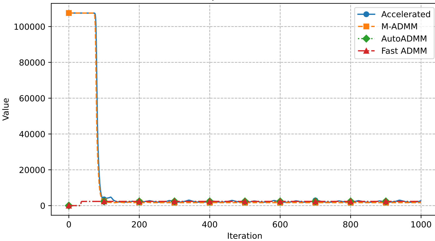
Primal Resid
