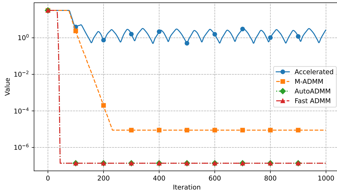
Primal Resid
