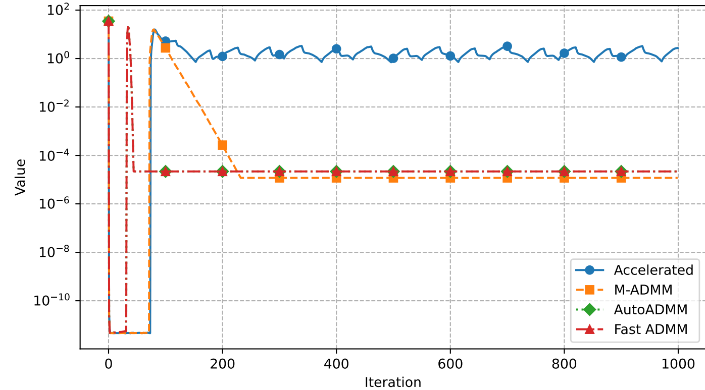
Dual Residuals
