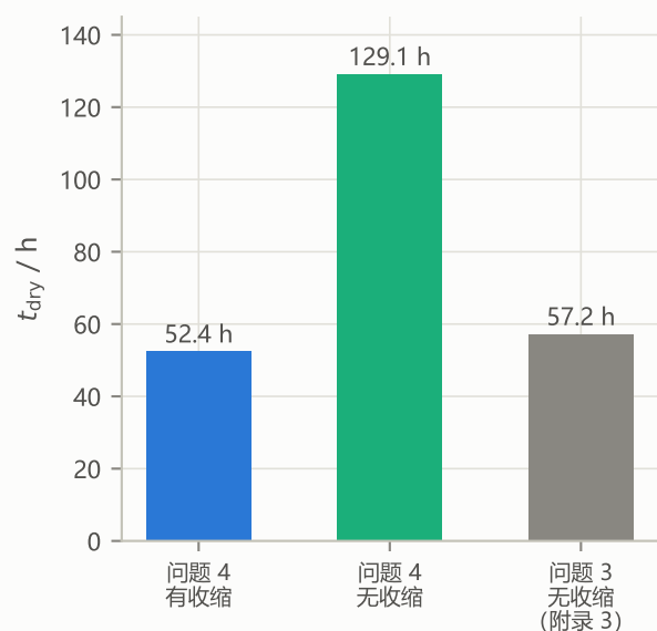
(c) 收缩对烘干时长的缩短
