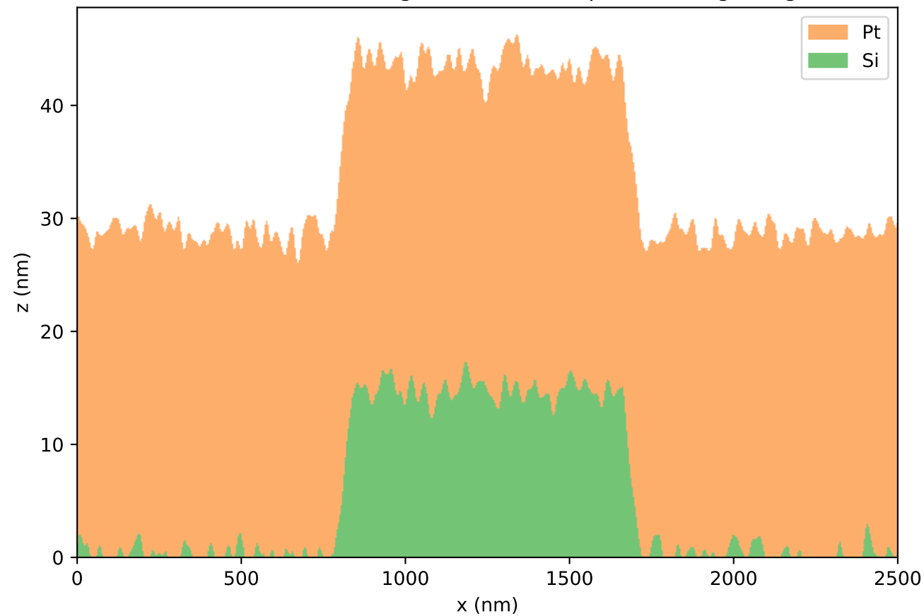
random-interface sigma=1.0 nm, supercells=3 grating
