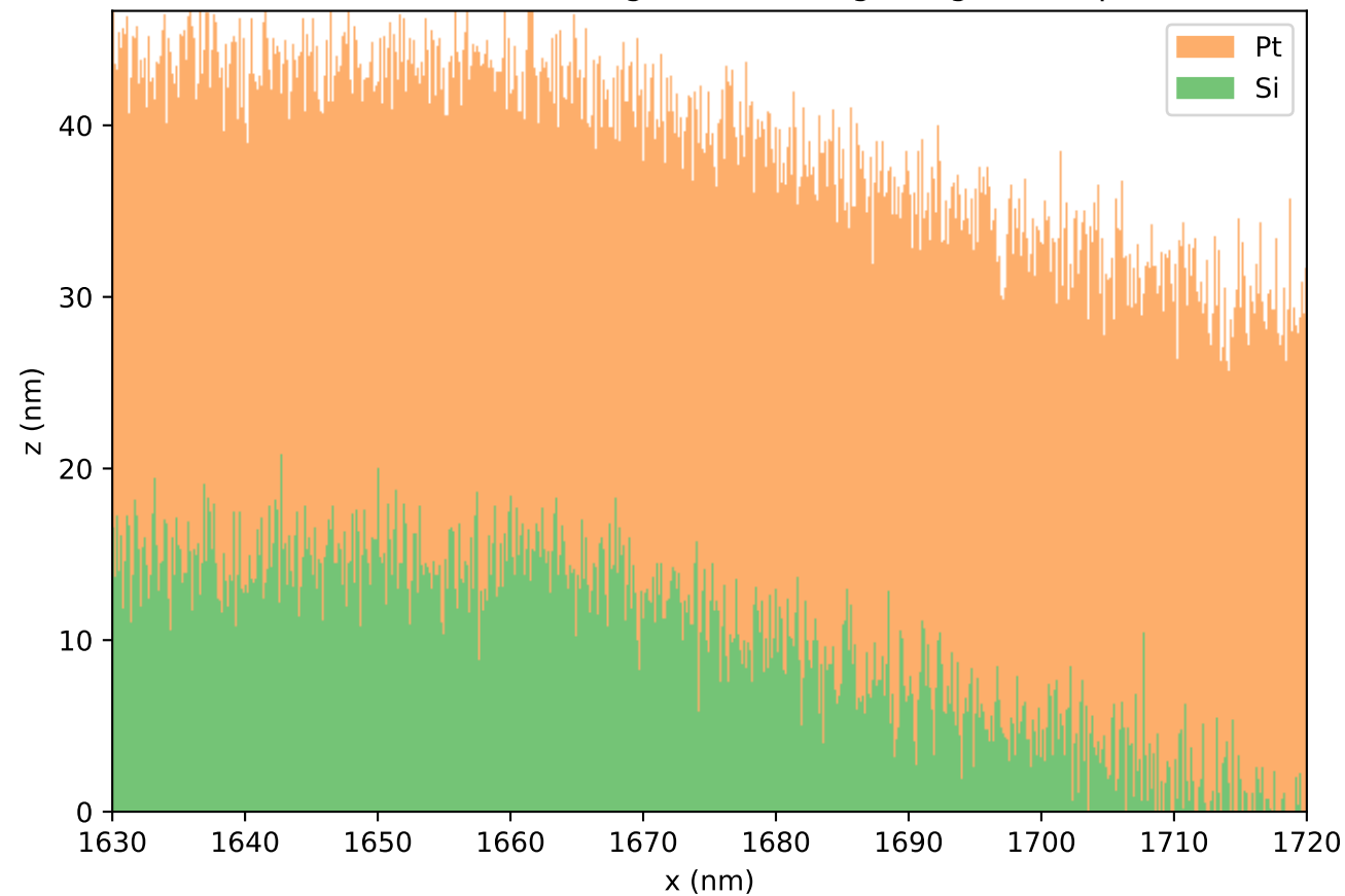
random-interface sigma=2.0 nm grating close-up
