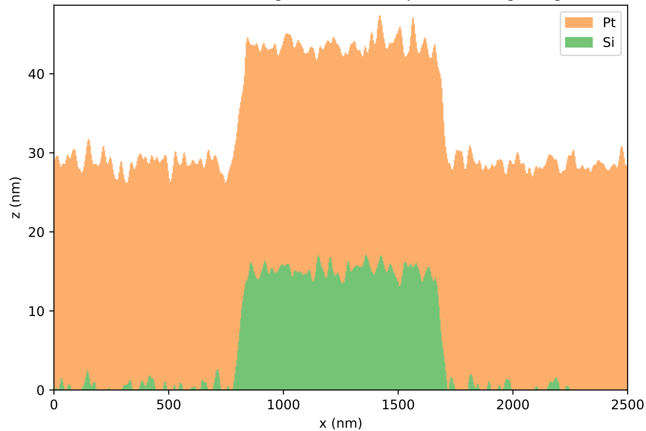
random-interface sigma=1.0 nm, supercells=10 grating
