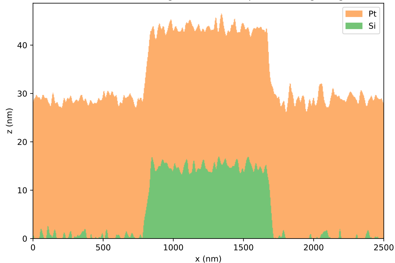
random-interface sigma=1.0 nm, supercells=30 grating
