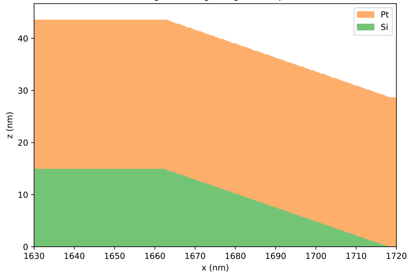
sigma zero grating close-up
