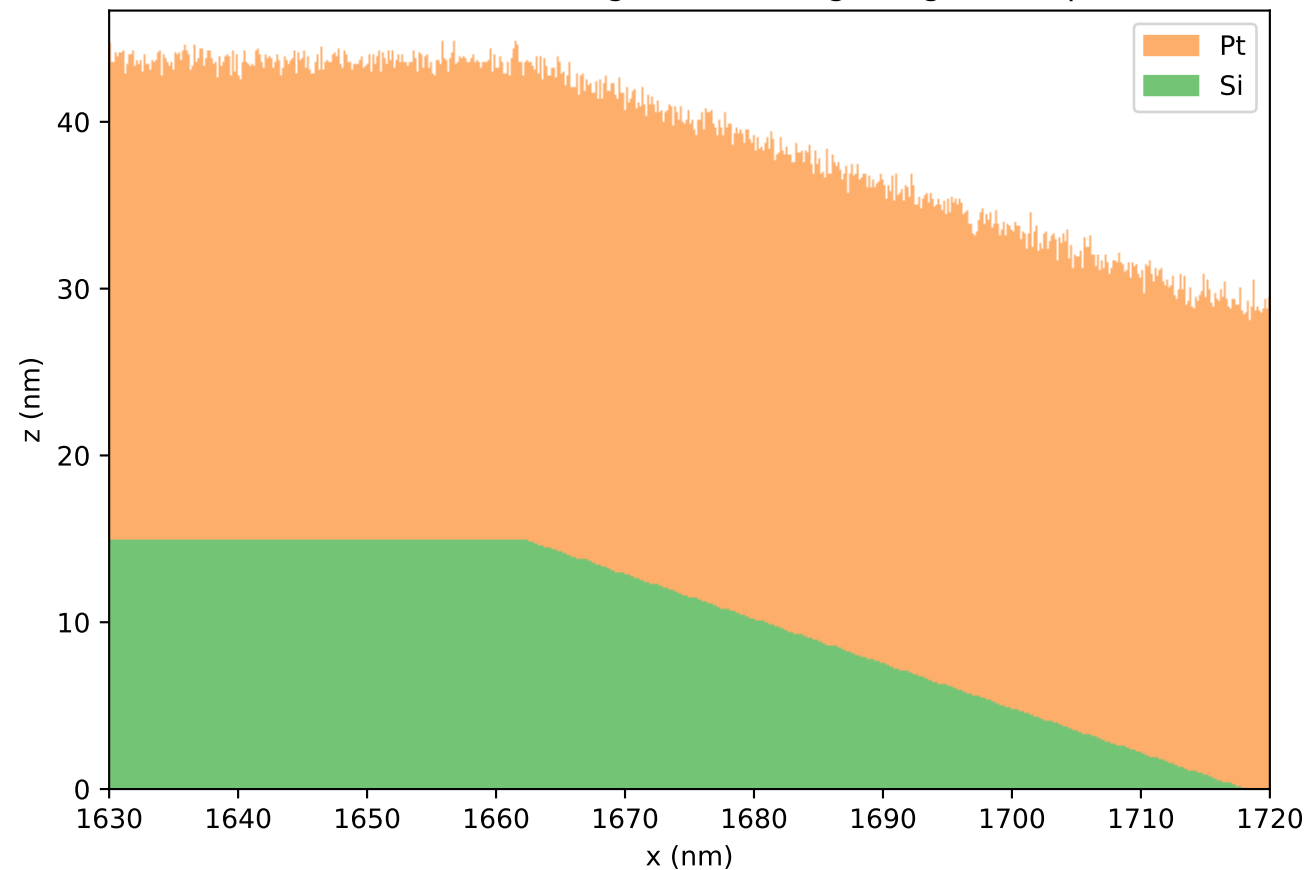
random-interface sigma=0.5 nm grating close-up
