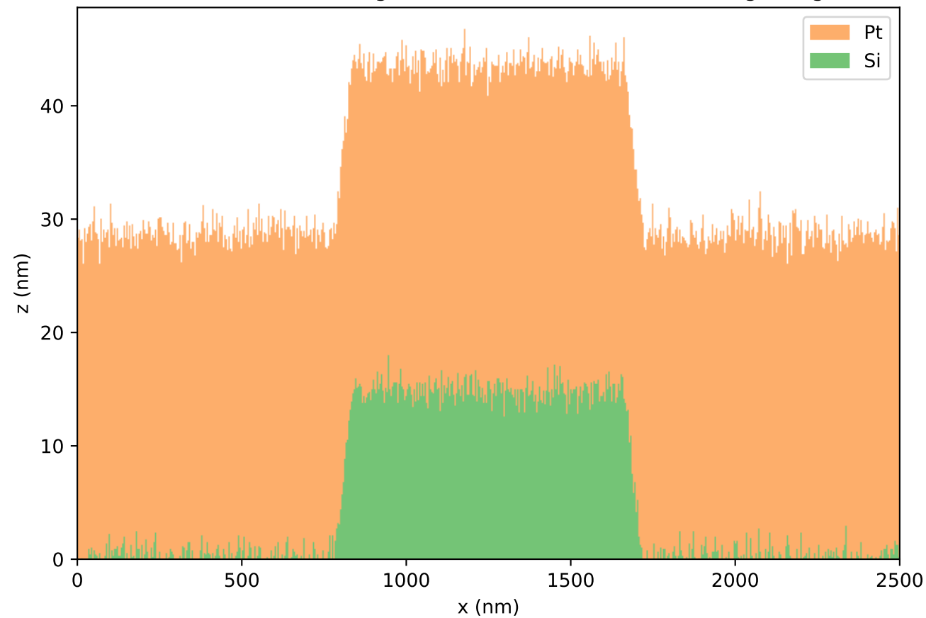
random-interface sigma=1.0 nm, correlation=0 nm grating
