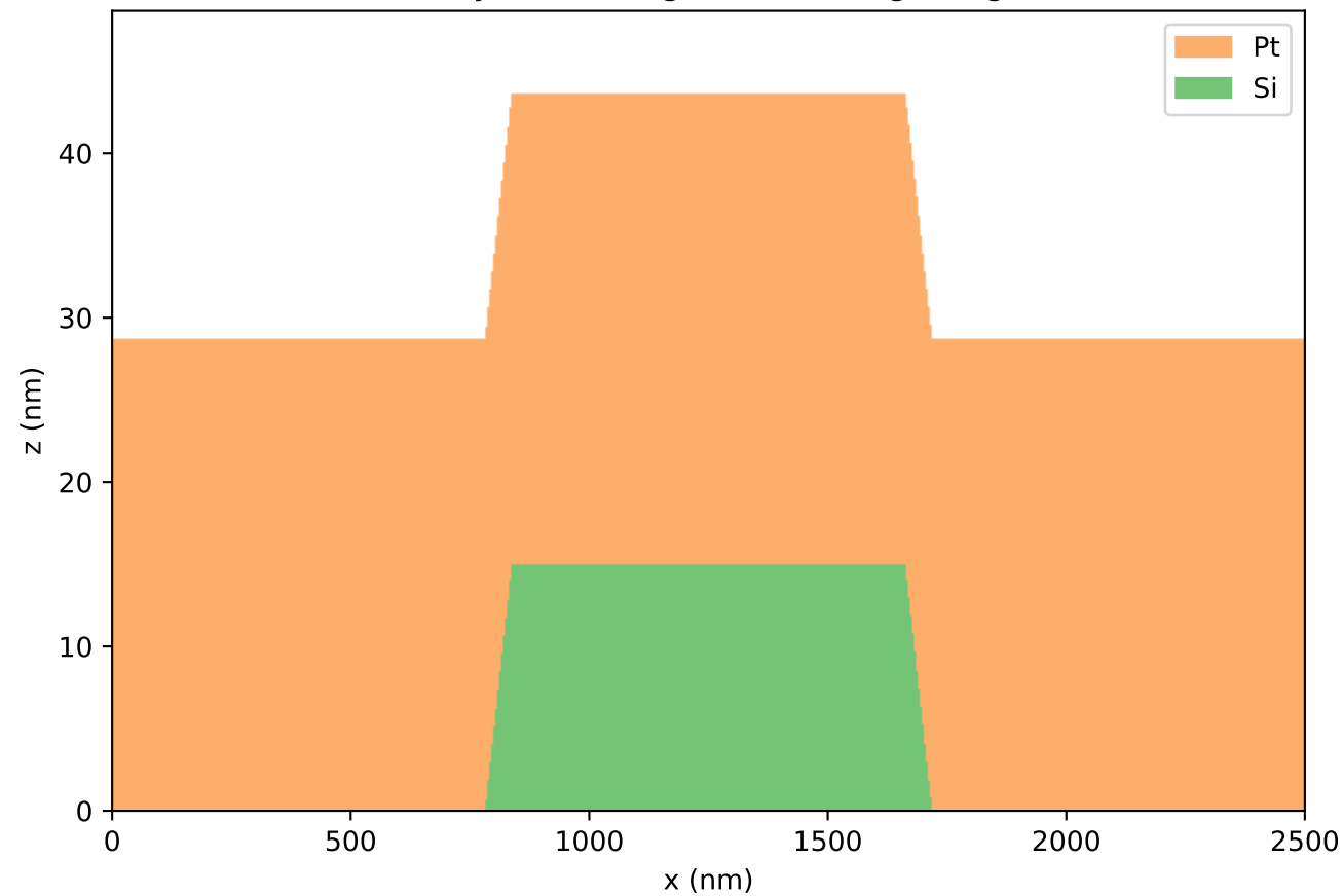
debye-waller sigma=1.0 nm grating
