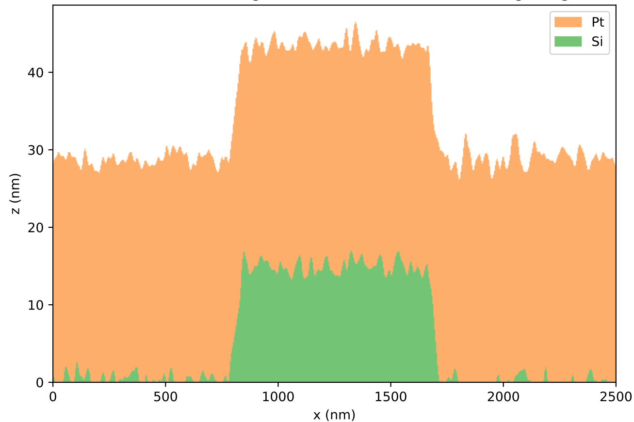
random-interface sigma=1.0 nm, correlation=10 nm grating
