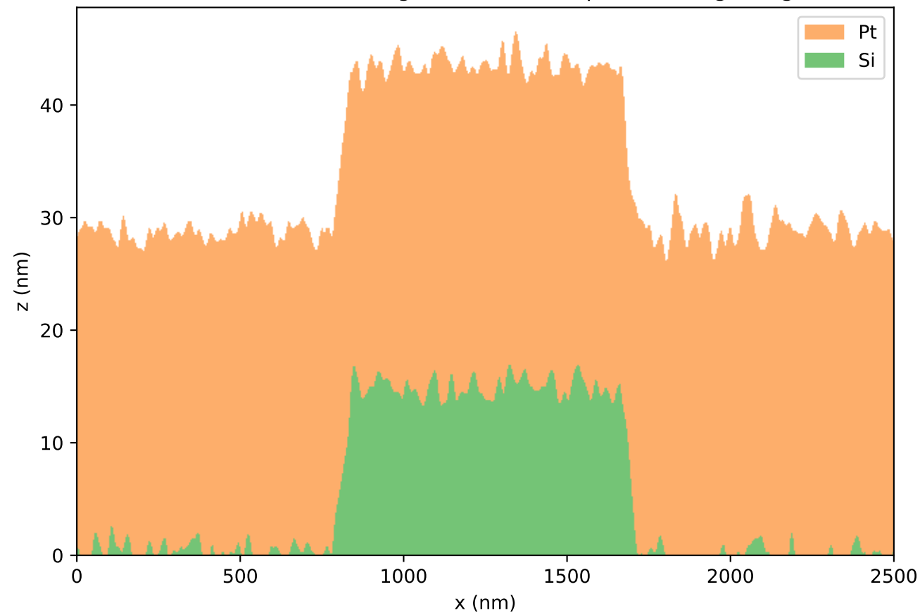
random-interface sigma=1.0 nm, supercells=5 grating
