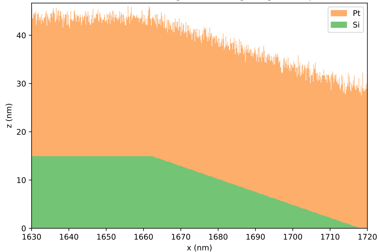
random-interface sigma=1.0 nm grating close-up
