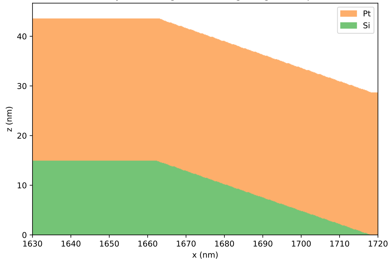
debye-waller sigma=1.0 nm grating close-up
