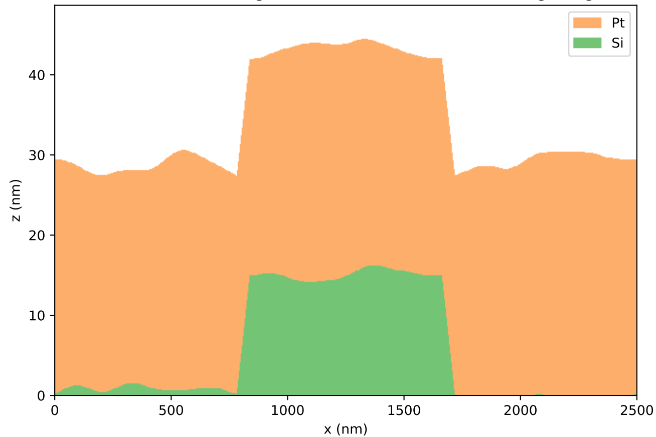
random-interface sigma=1.0 nm, correlation=100 nm grating
