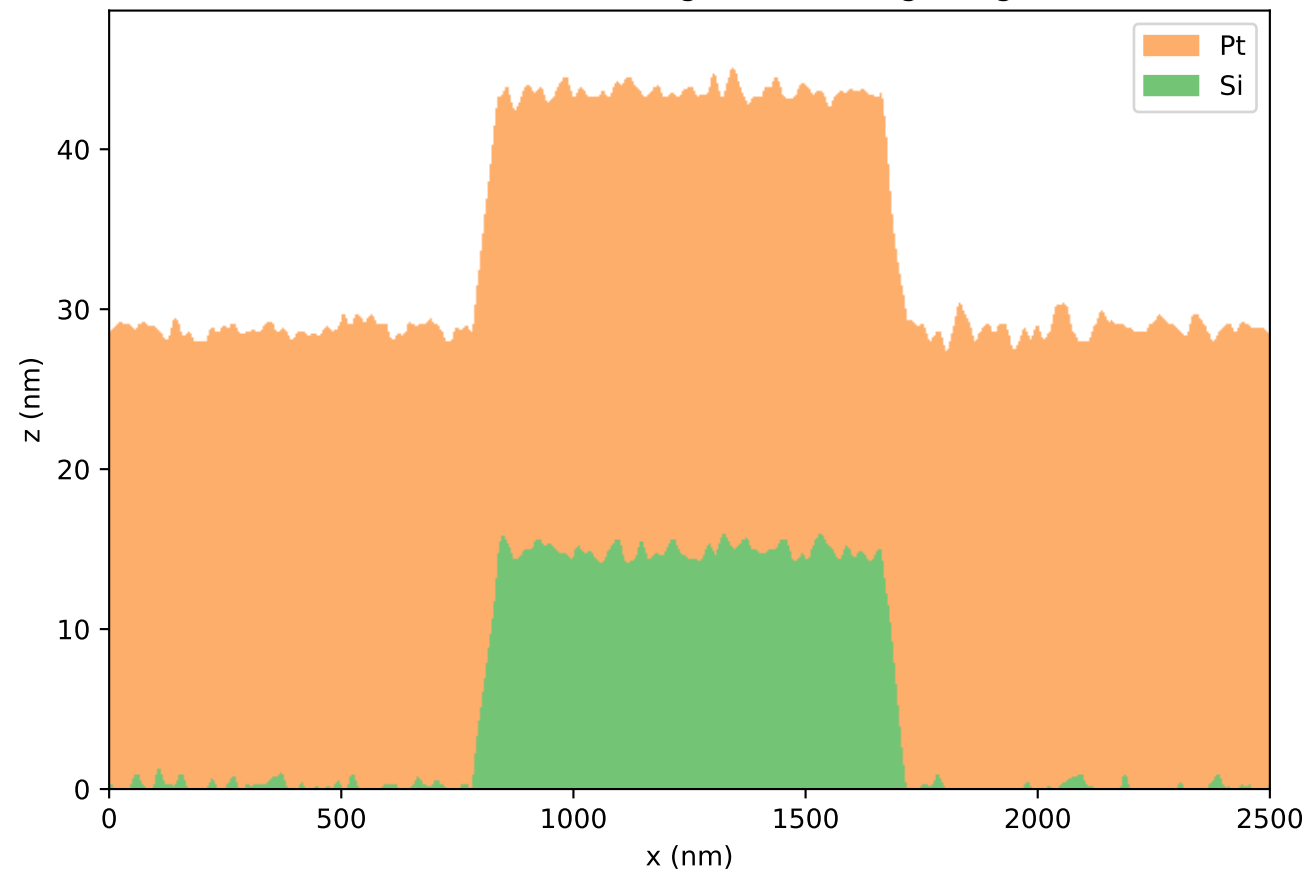
random-interface sigma=0.5 nm grating
