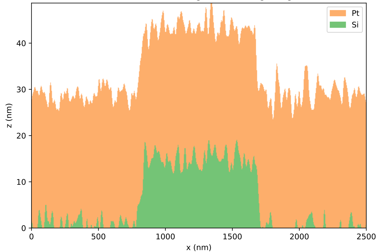
random-interface sigma=2.0 nm grating
