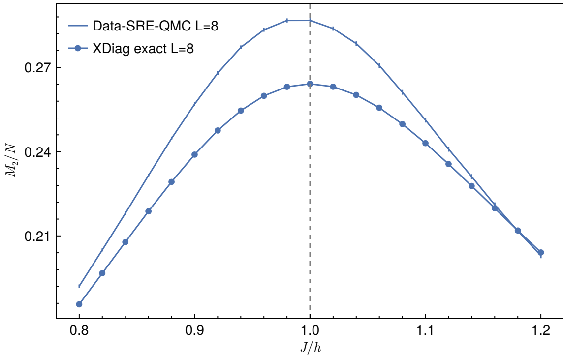
Exact Ising vs Data-SRE-QMC, N = 8
