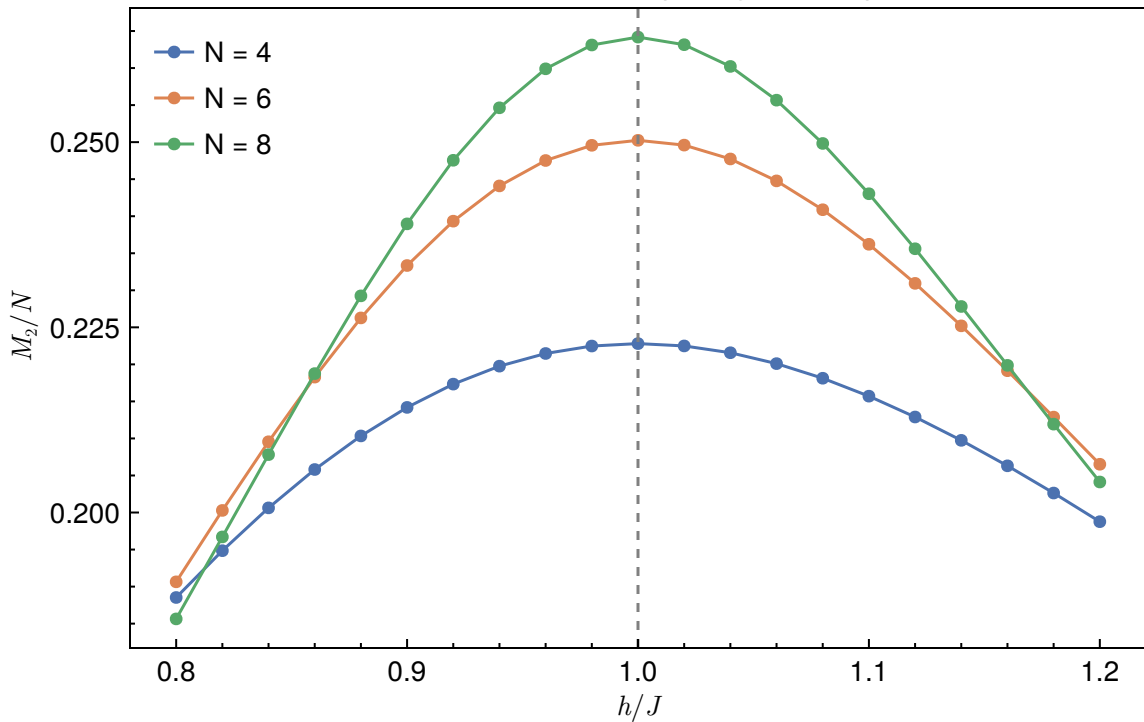
Exact stabilizer Rényi magic density
