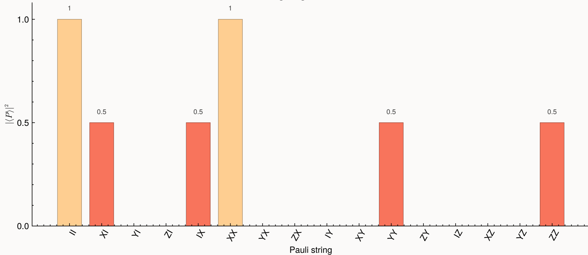
TFIM Pauli-string weights, N = 2 , h = 1.0 , J = 1.0
