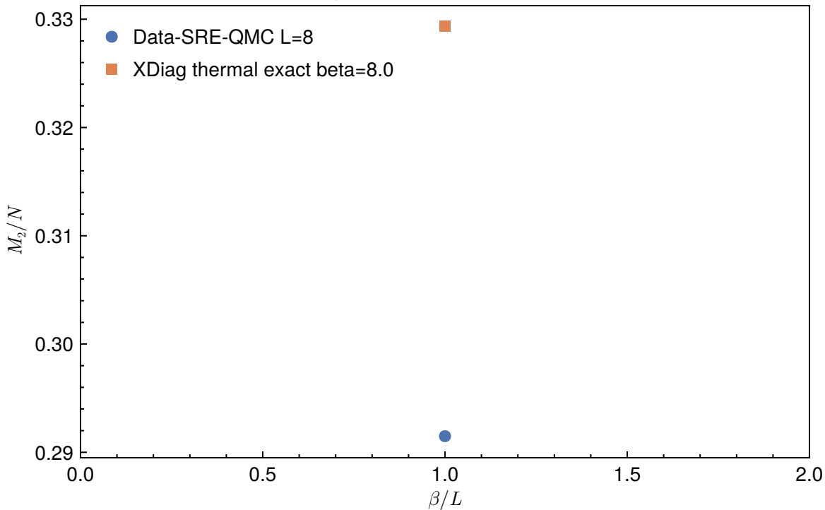
Thermal Ising vs Data-SRE-QMC, L = 8, beta = 8.0
