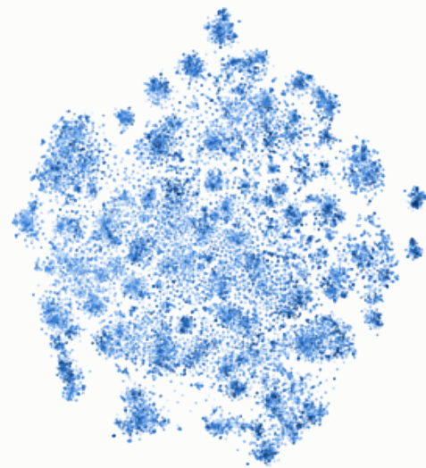
(c) t-SNE
