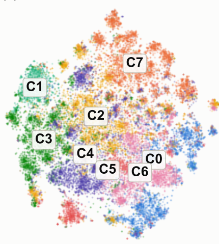
(c) t-SNE
