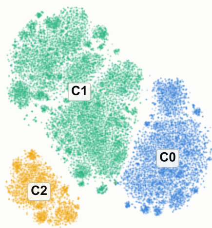
(c) t-SNE
