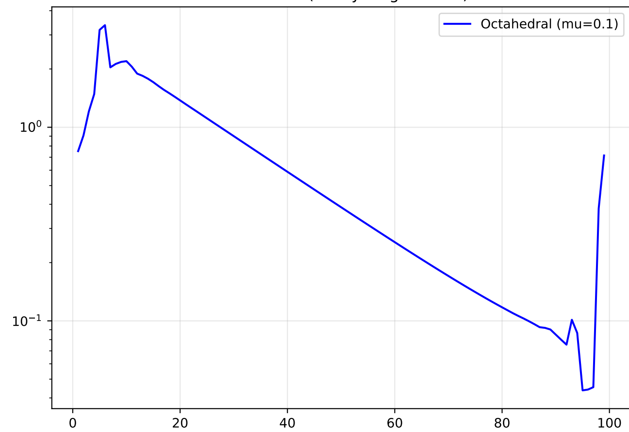
Weak Force (decay length=30.0)
