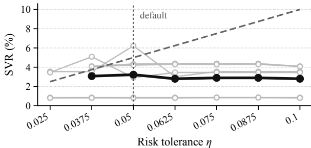
(b) Held-out SVR
