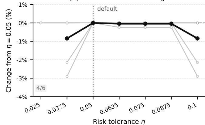
(a) Normalized cost change
