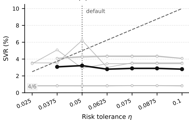
(b) Held-out SVR
