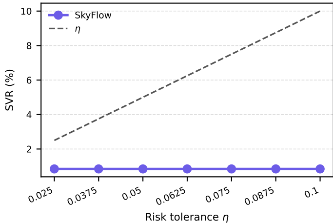
workflow1 Q2: SVR
