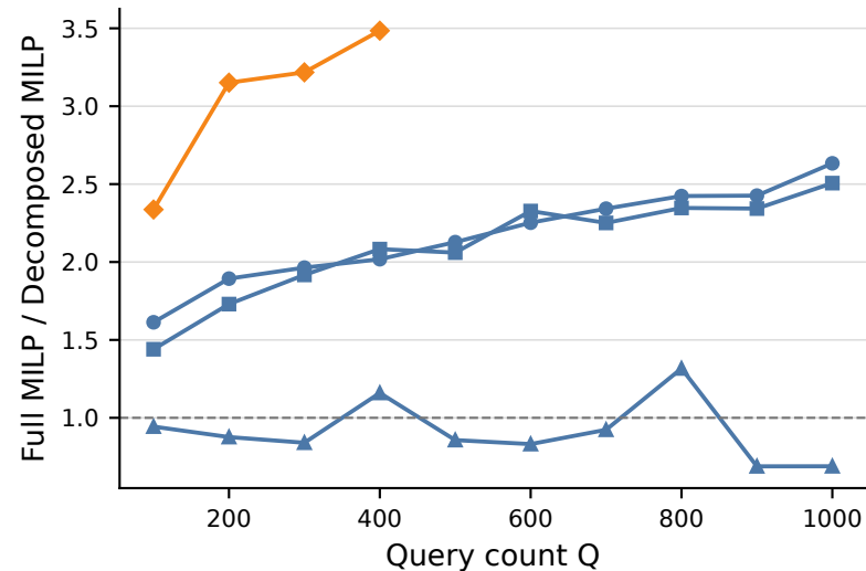
Runtime Ratio
