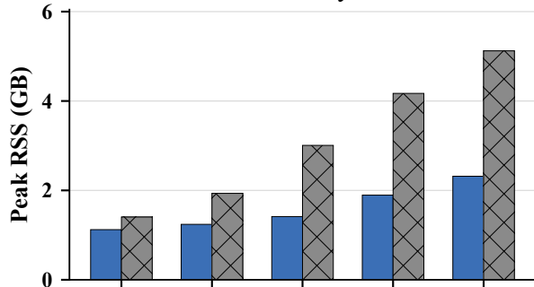
Memory
