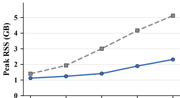
Memory
