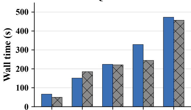
W2-Q1 Runtime
