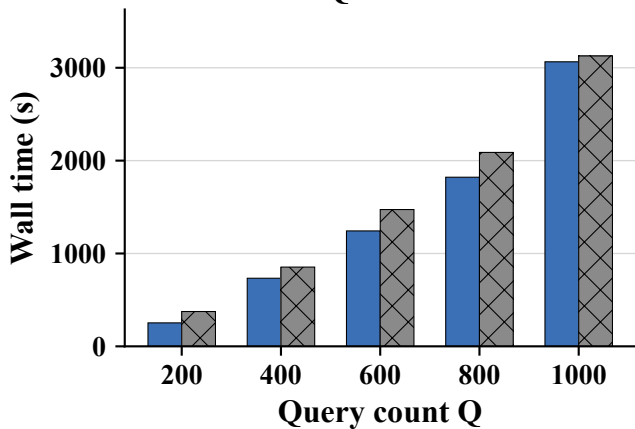
W2-Q1 Runtime
