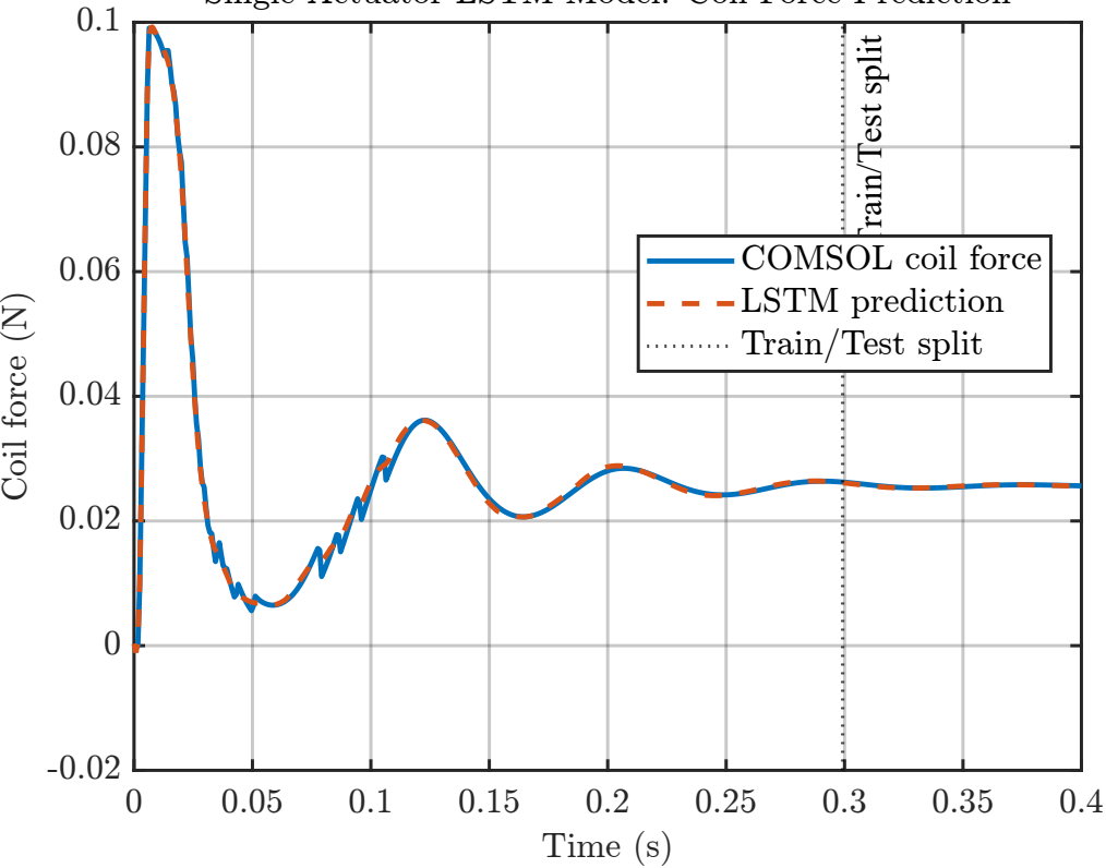
Single Actuator LSTM Model: Coil Force Prediction
