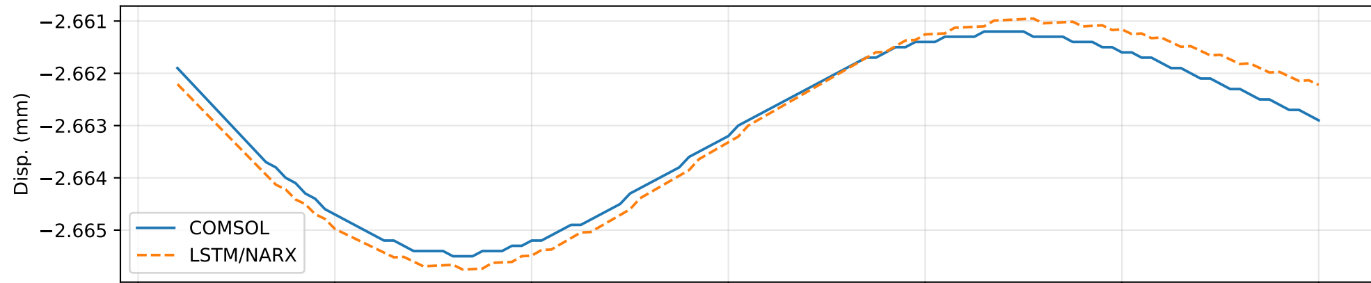
Displacement: RMSE=0.0003033 mm, R2=0.9571
