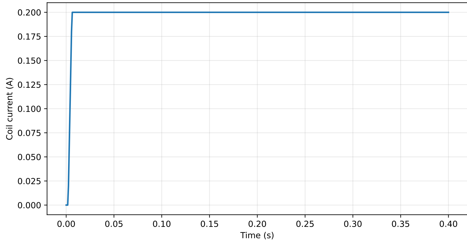
Input Current Profile for Single ESA Actuator
