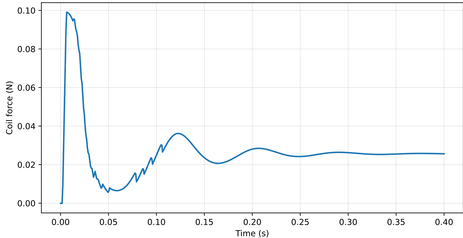
Electromagnetic Coil Force Response
