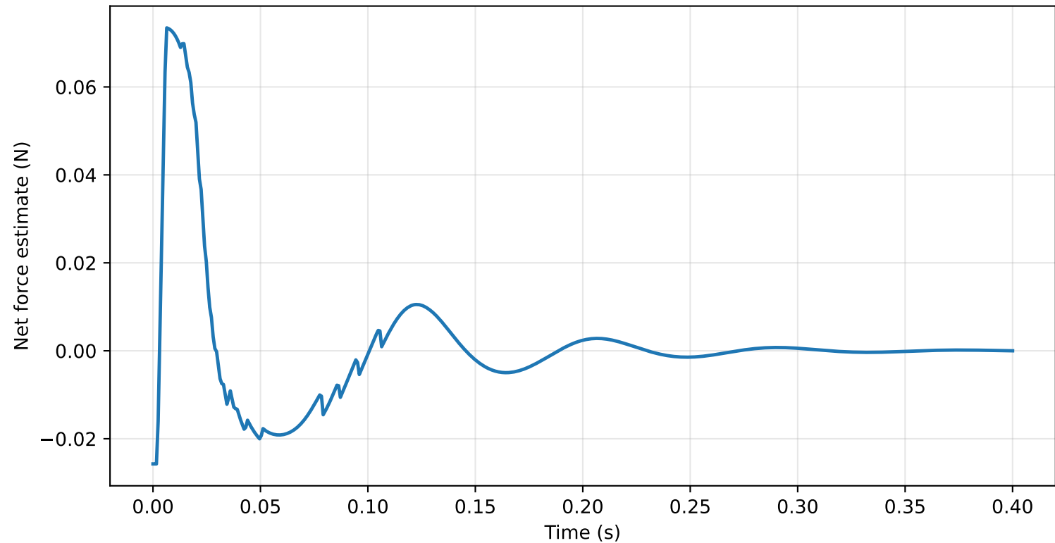
Net Force Estimate: Coil Force Minus Weight/Load
