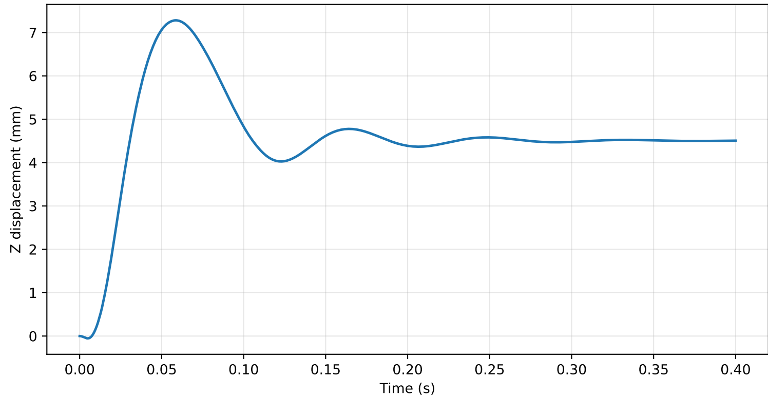
Z Displacement Response of Single ESA Actuator
