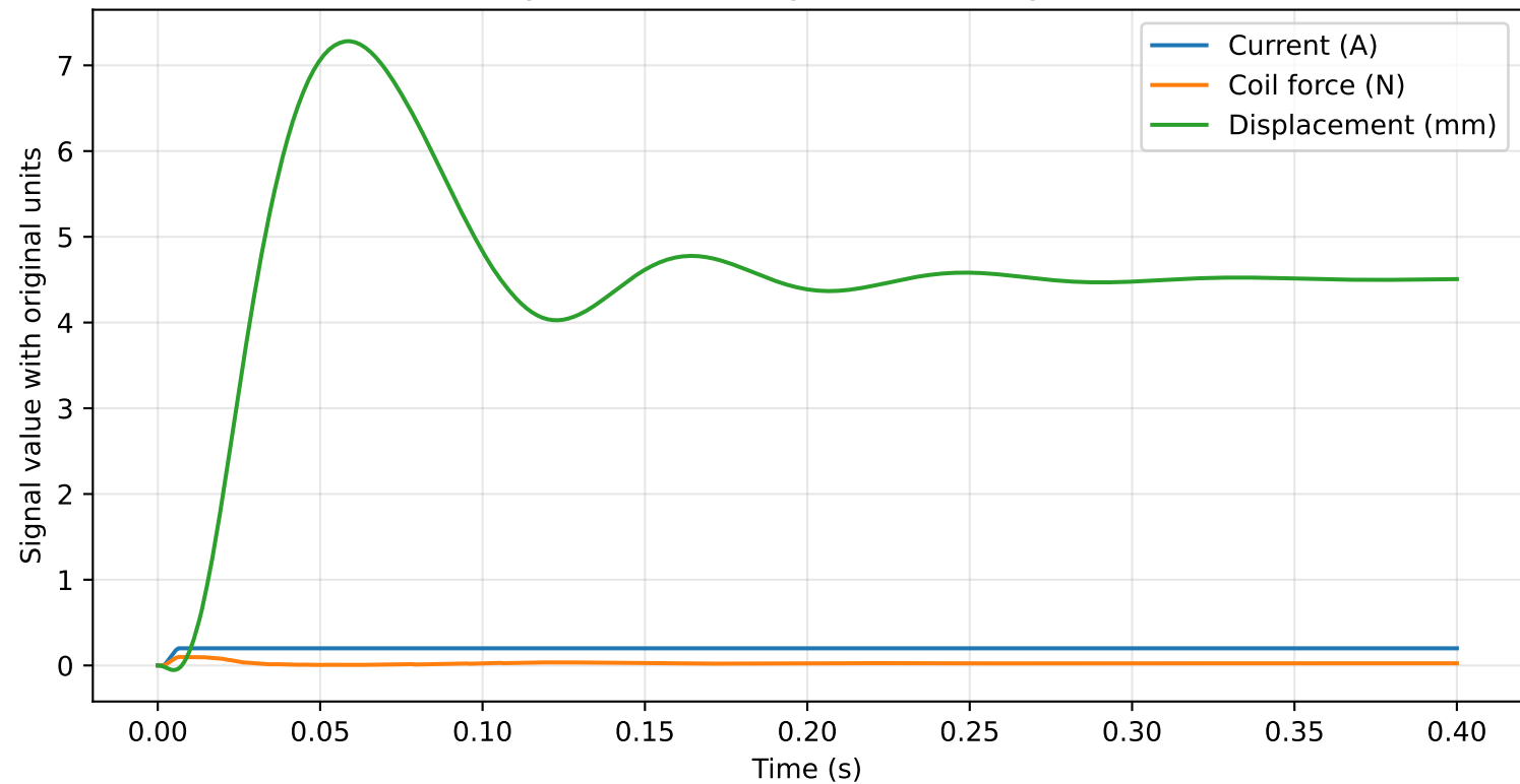
Synchronized Single Actuator Signals
