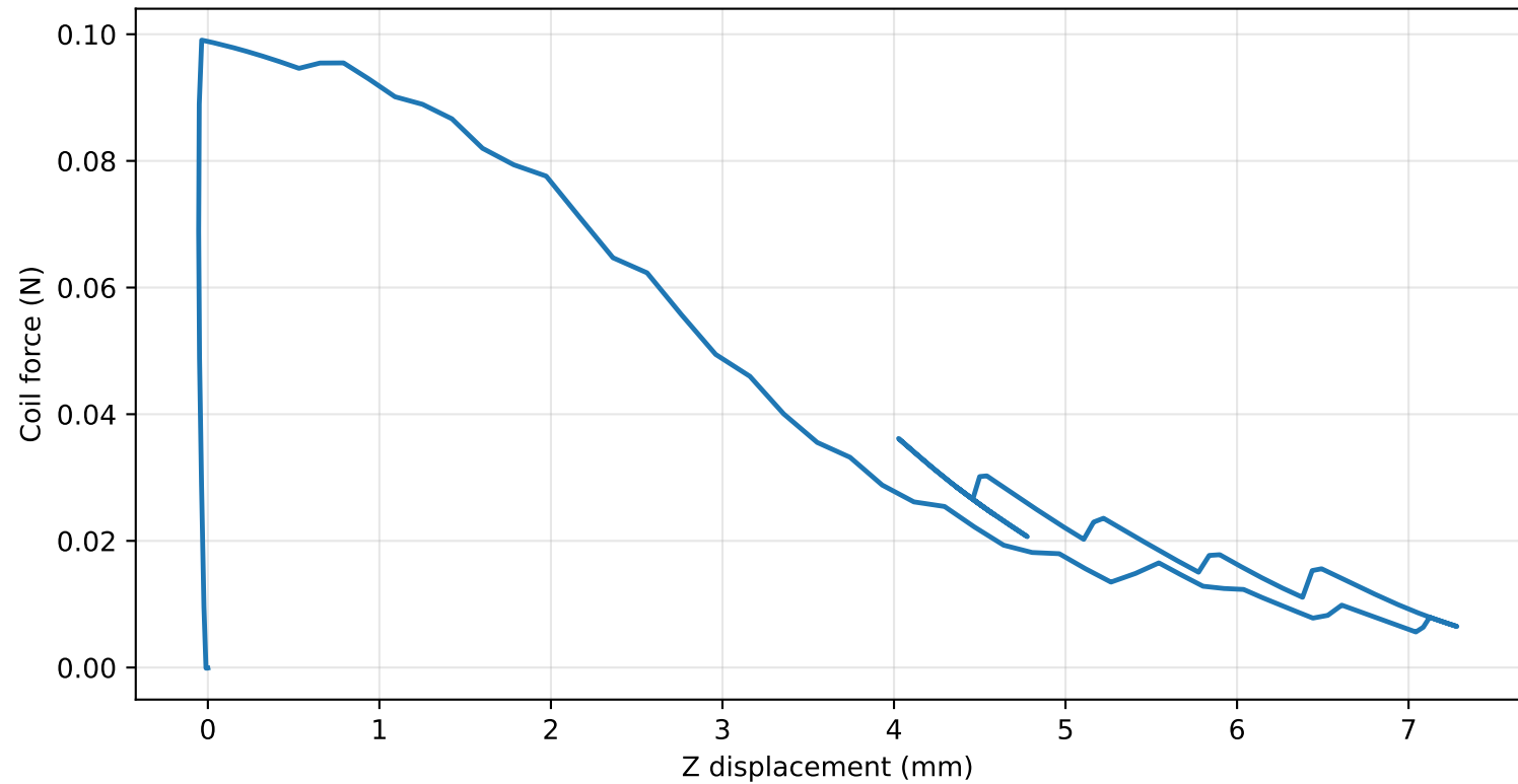
Force Versus Displacement
