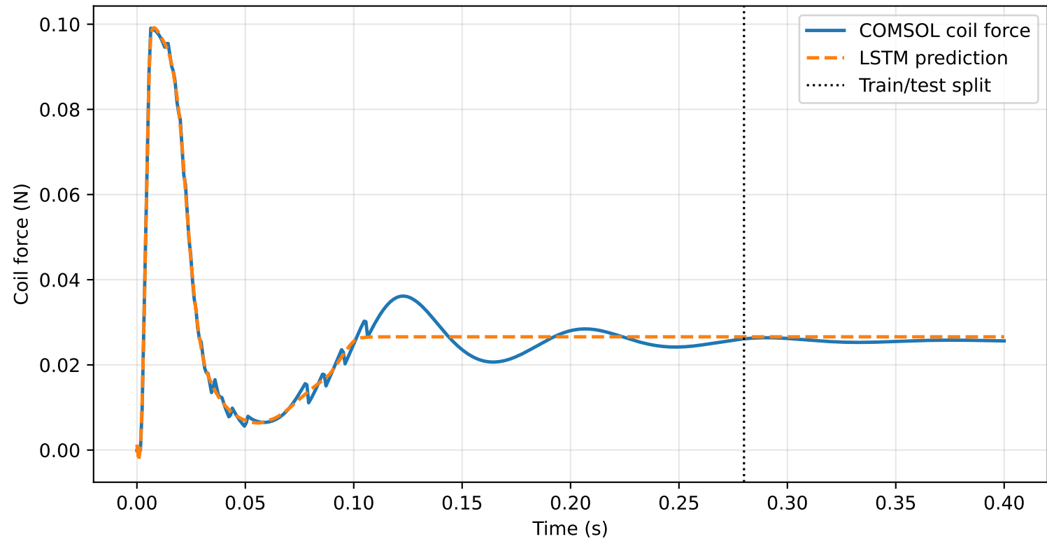
Single Actuator LSTM Model: Coil Force Prediction
