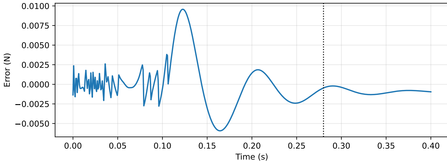
Coil Force Prediction Error: COMSOL minus LSTM
