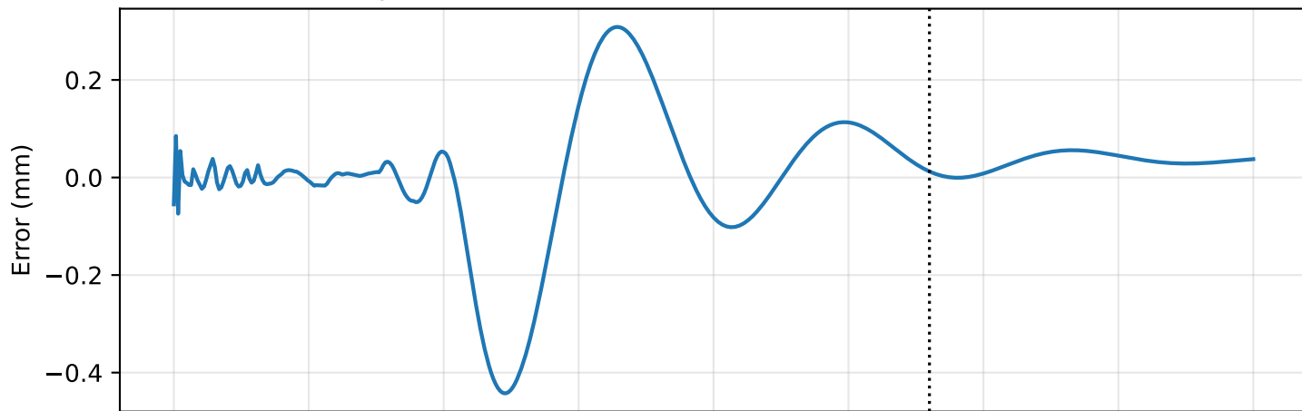
Displacement Prediction Error: COMSOL minus LSTM
