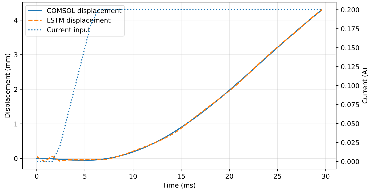
Early Transient: Current Trigger and LSTM Displacement Prediction
