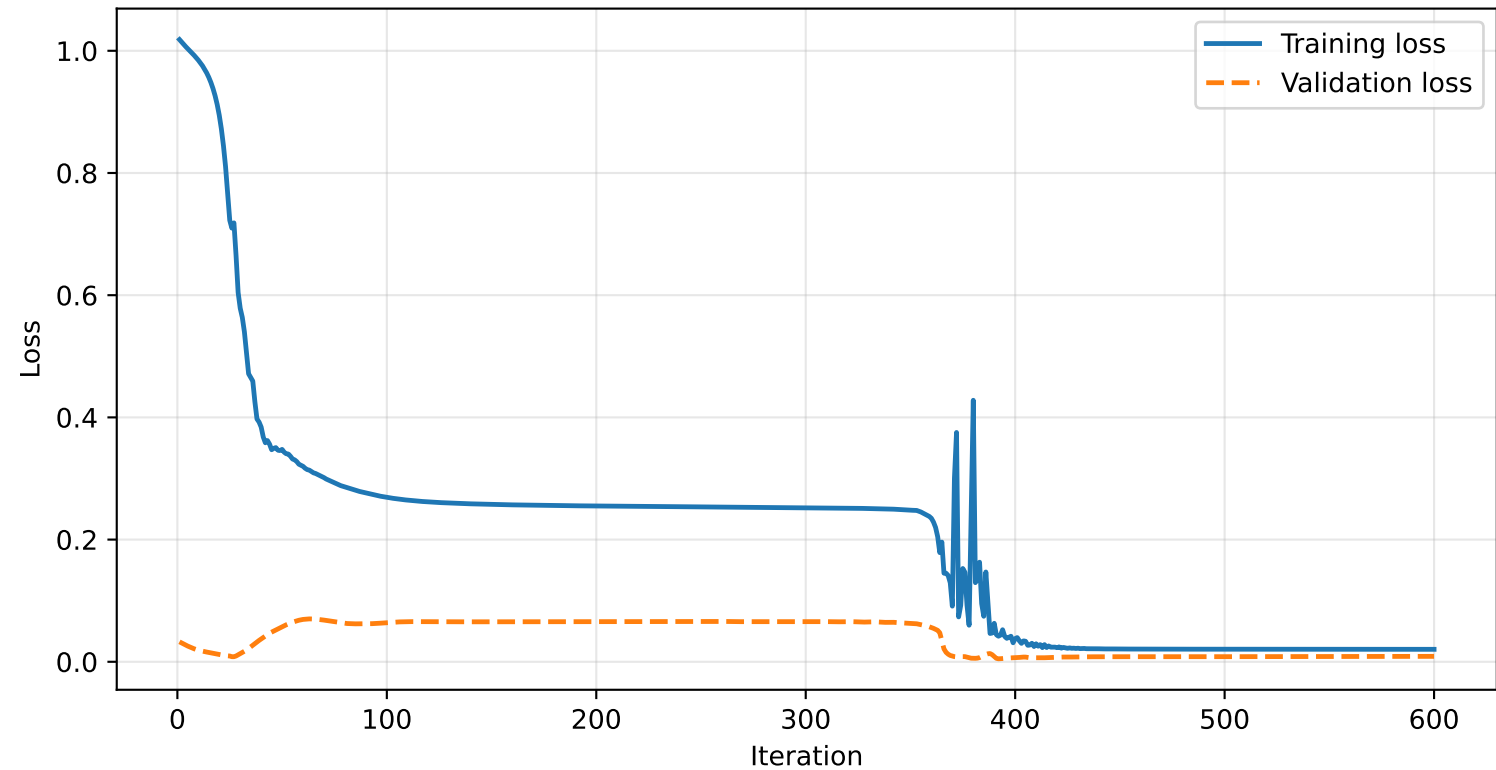
LSTM Training and Validation Loss History
